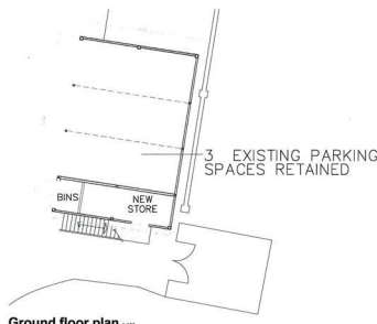
Ground floor plan 1:100
